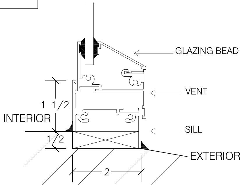
RL2 ALUMINUM PROJECTION & CASEMENT WINDOWS ODD LEG FRAME
