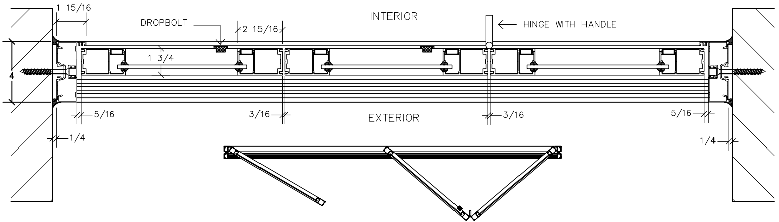
OPENING OF BIFOLD DOOR
