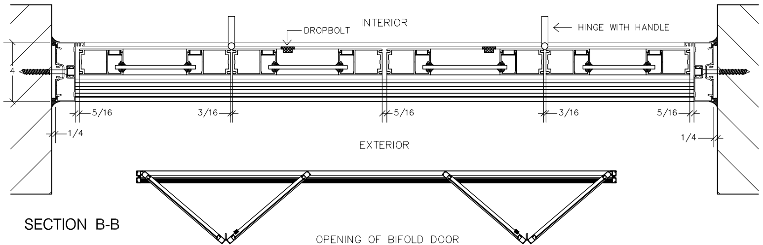
OPENING OF BIFOLD DOOR
