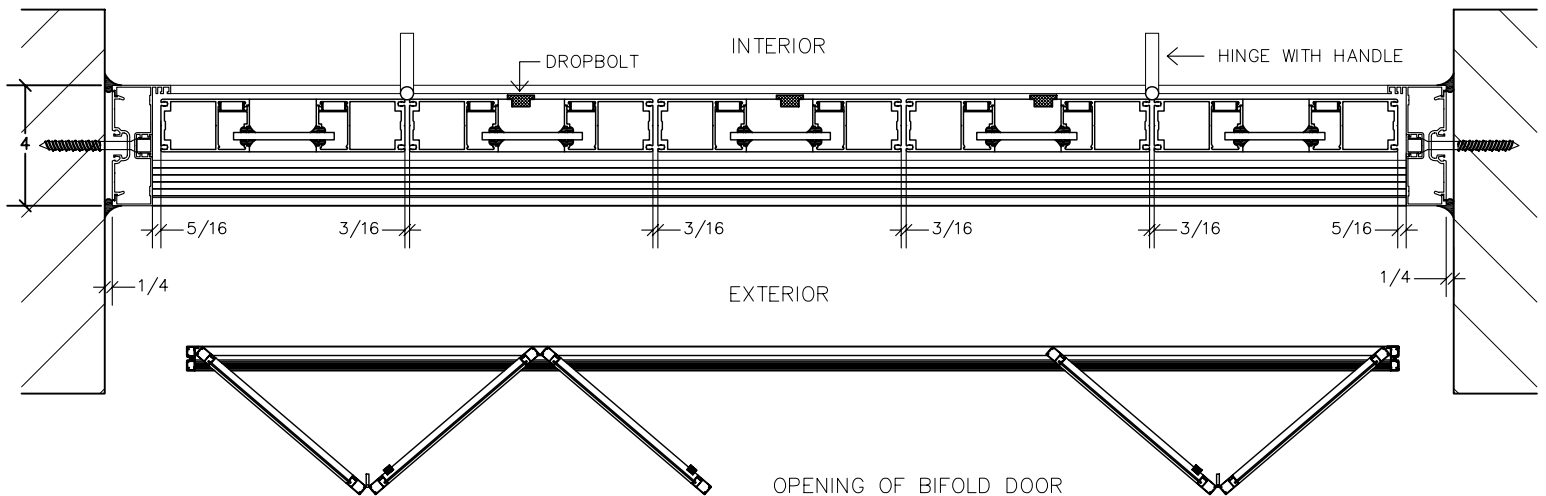
SECTION C-C
