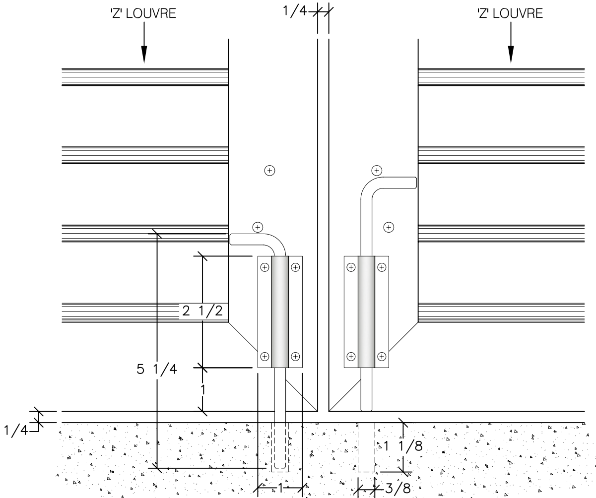
SECTION C DETAIL OF SLIDER BOLT
