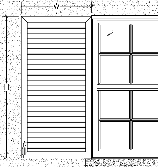
ALUMINUM 'Z' LOUVRE SHUTTERS (OPEN)
