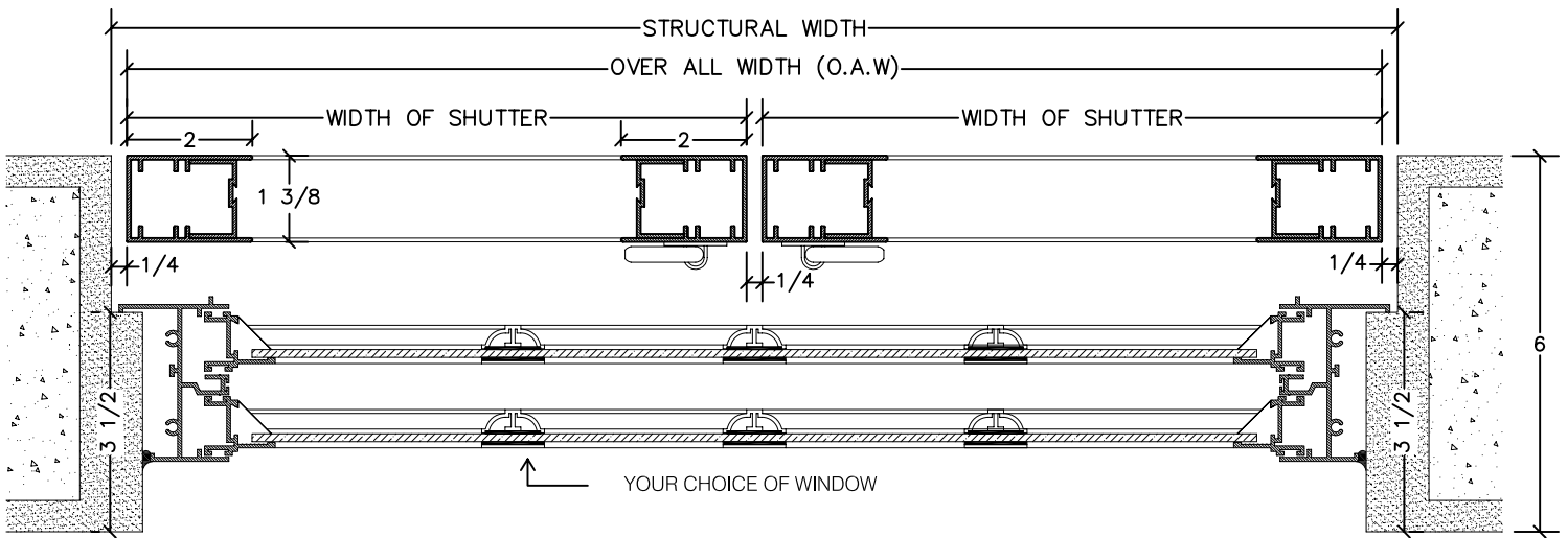
SECTION B-B
