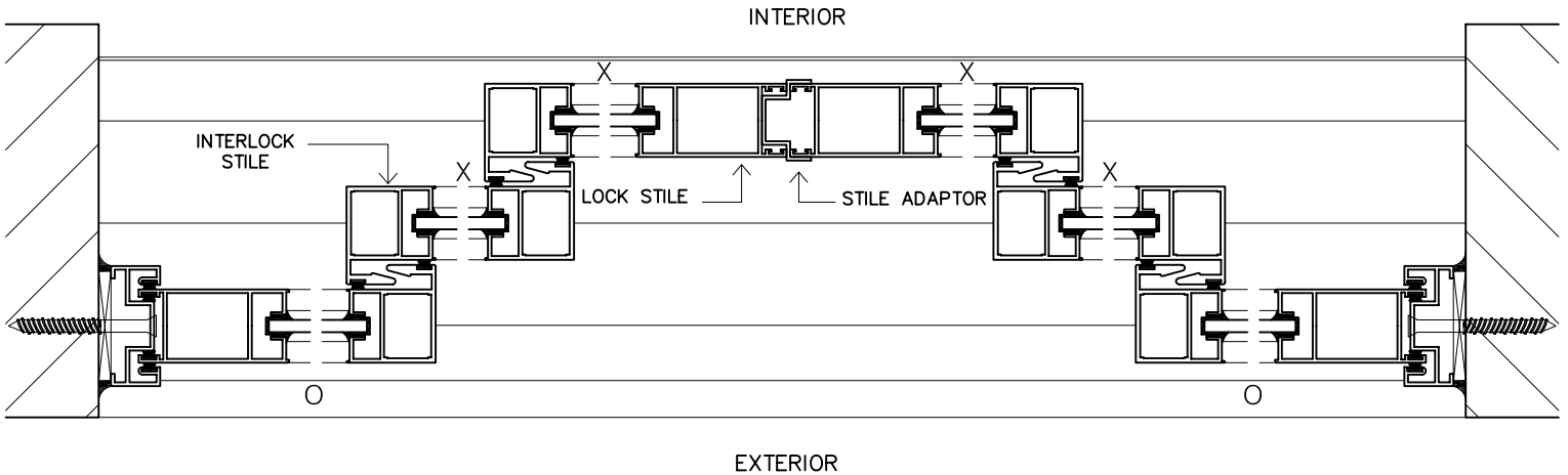
SECTION C-C
